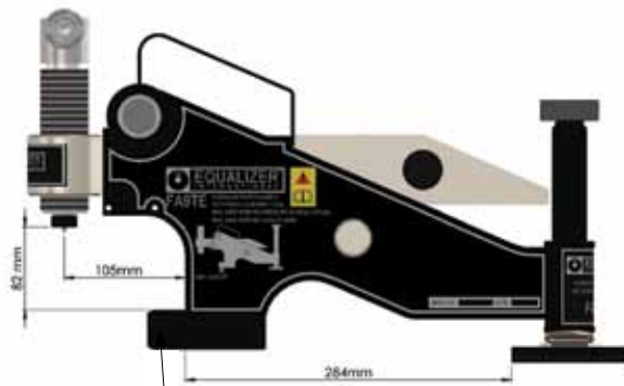
Minimum Extension
