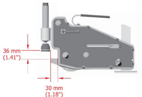
Minimum extension
