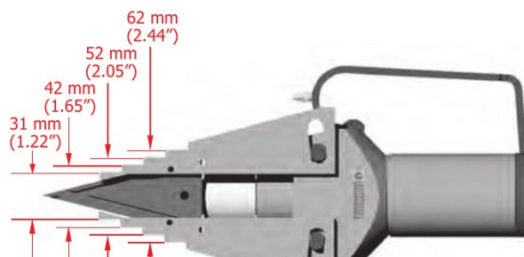
Tool open
