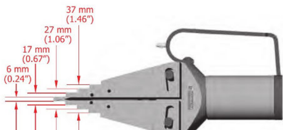
Tool closed
