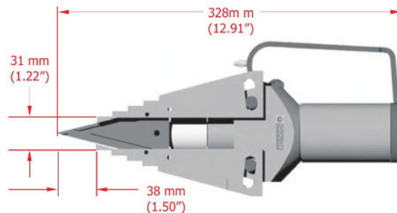
Tool open
