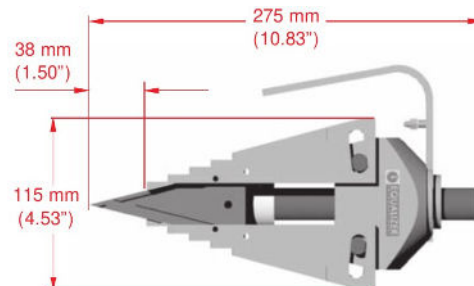
Tool open
