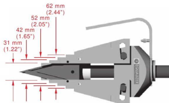
Tool open
