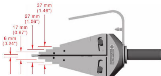
Tool closed
