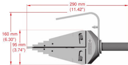
Tool closed
